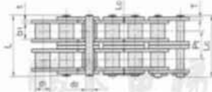
FF0424 扶梯三排链条 Escalator third row chain
